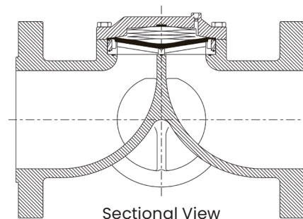
Sectional View
