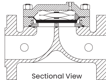
3" Single Port Valve with Series 20 Pilot
